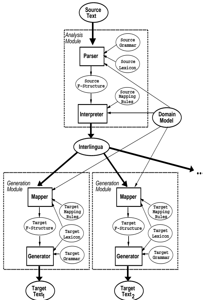
Figure 2: KANT: Knowledge-Based Natural Language Translation
